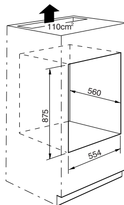
PROUD MOUNT CUTOUT
