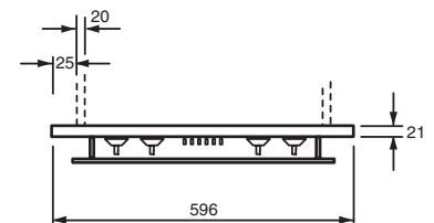
PLAN (FRONT)
