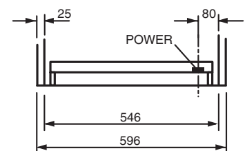
REAR (LOWER) ELEVATION POWER
