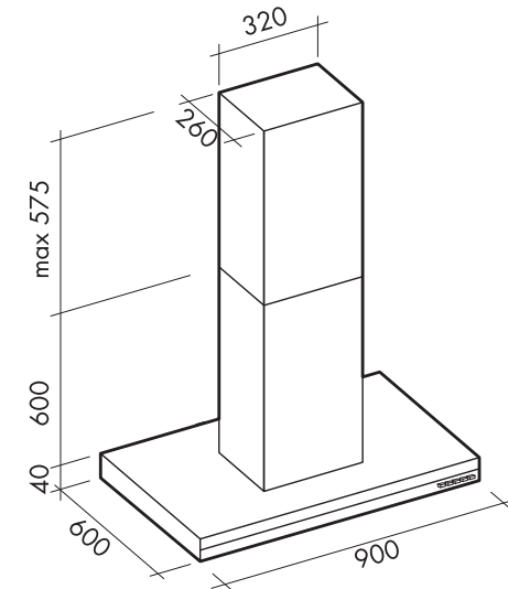
BHH9034 - IS : FLUE OUTLET - 150MM CARBON FILTER - GECF0113 FLUE COVER EXTENSION - GEFE1200
