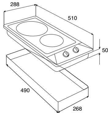
BACE3036-P : HARD WIRED 15 AMP
