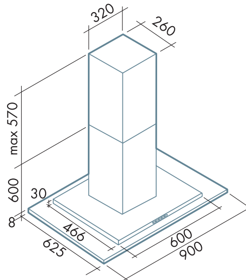
BHH9029G-IS : FLUE OUTLET - 150MM CARBON FILTER - GECF0113 FLUE COVER EXTENSION - GEFE1200
