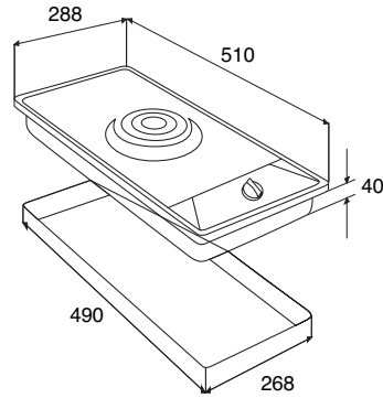
BACG3035-P : 10 AMP PLUG
