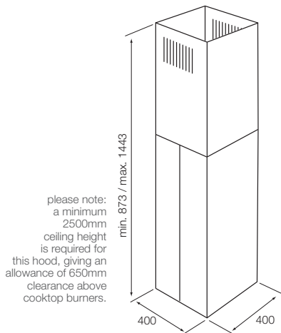
BAH4030-P : FLUE OUTLET - 150MM CARBON FILTER - GECF0114
