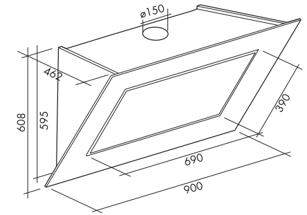
BAH9031-P : FLUE OUTLET - 150MM CARBON FILTER - GECF0114
