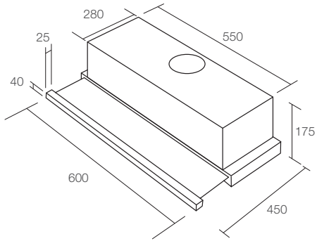
BAH6018 : FLUE OUTLET - 120MM CARBON FILTER - GECE0107
