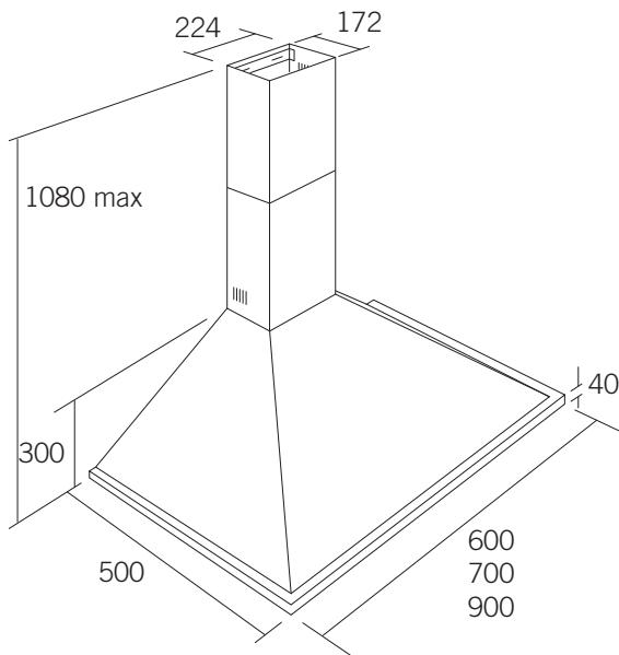
BAH9007 + BAH6008 + BAH7006 : FLUE OUTLET - 120MM CARBON FILTER - GECE0108 FLUE COVER EXTENSION - GEFE1202
