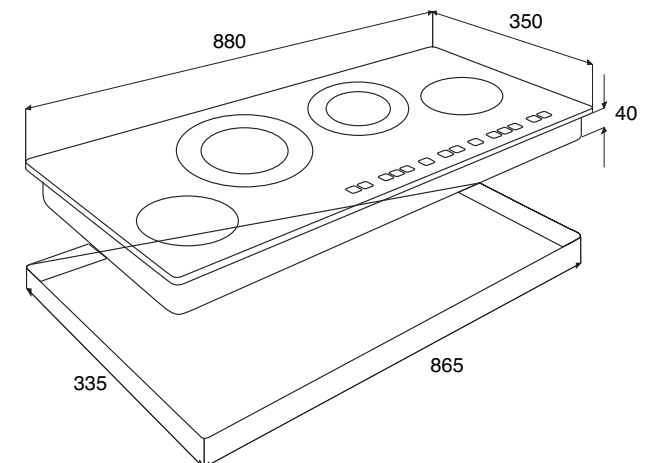
BACE9001 : HARD WIRED 30 AMP
