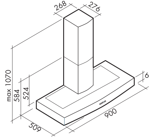
BHH9035 : FLUE OUTLET - 150MM CARBON FILTER - GECF0113 FLUE COVER EXTENSION - GEFE9605
