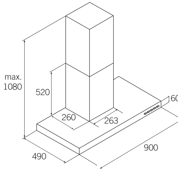
BHH9028 : FLUE OUTLET - 150MM CARBON FILTER - GECE0113 FLUE COVER EXTENSION - GEFE9602
