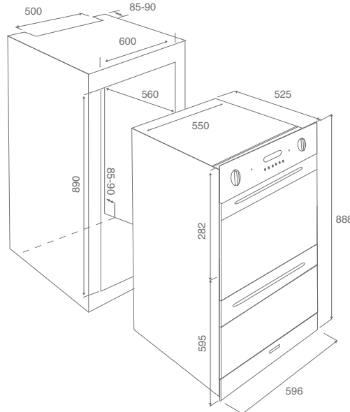
BAO6008-P : HARD WIRED 30 AMP
