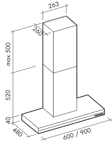
BHH9034 : FLUE OUTLET - 150MM CARBON FILTER - GECF0113 FLUE COVER EXTENSION - GEFE9602
