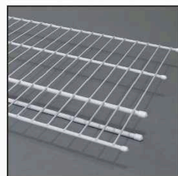
Shelf & Rod 400/250 S & R 400mm deep, hanging rail 250mm from wall (for wardrobes less than 550mm deep) 400/300 S & R 400mm deep, hanging rail 300mm from wall (for wardrobes more than 550mm deep)
