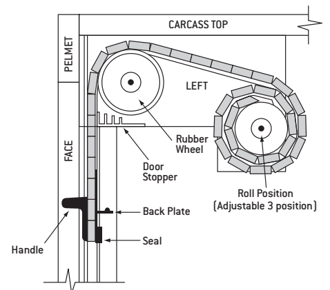
• Cross Sectional diagram of roller shutter unit.
